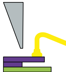
Figure 1. Alignment of shear tool with ball bond
