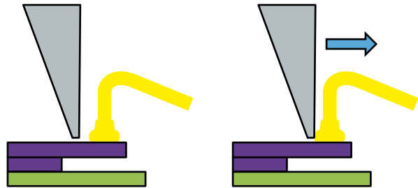
Figure 4. Step back of the shear tool followed by bond shear
