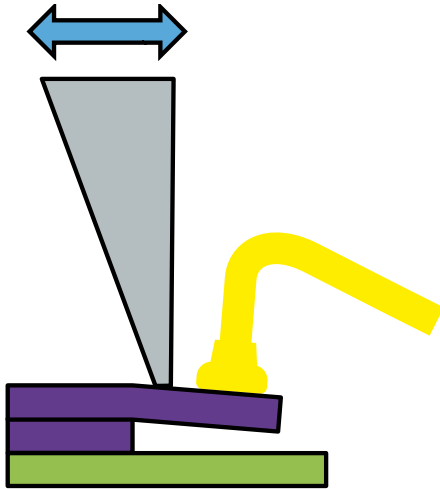
Figure 2. Shear tool lands and oscillates producing a measurable force on the transducer
