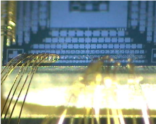
Figure 5. Typical view as seen through a stereomicroscope with 128X optics and 0.2mm FOV
