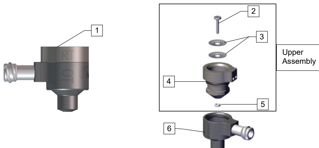
Figure 1-2 RT Jet Cartridge
