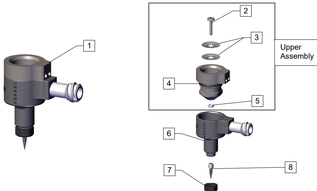
Figure 1-1 RT Stinger Cartridge Components
