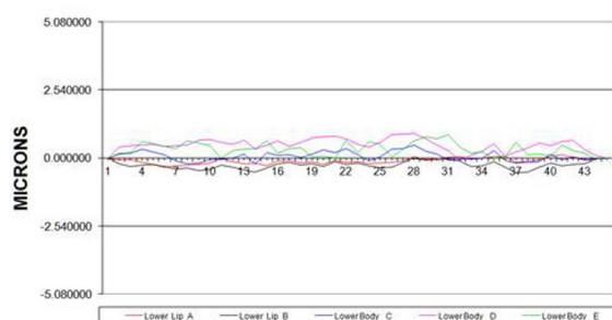
FLATNESS INSPECTION REPORT
