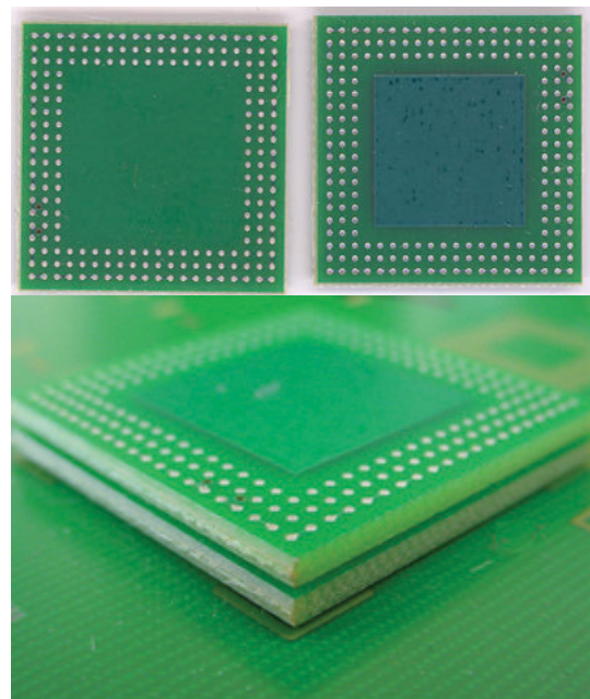
Picture 1: Optical images of the individual elements and a 'manufactured' example of a 'home-made' POP device. These home-made packages were made using the DEK balling process with solder spheres and tack flux provided by Indium Corp.
