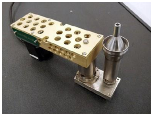
ControlFlow system with grooved riser and sleeve
