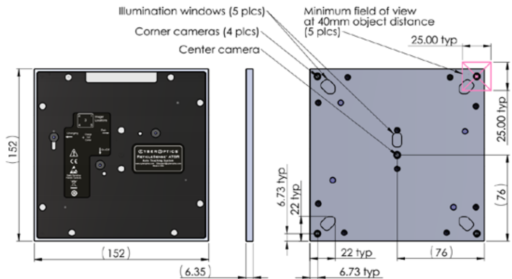
Figure 5 The new reticle-like teaching sensor has five downward-looking, high-resolution, color cameras, one in the center and one at each corner. The ATSR housing is machined from a quartz plate with a glass cover retaining the internal optics and electronics. The reticle shape conforms to the 6-inch SEMI reticle standard. The figure shows top (left) and bottom (right) views of the ATSR.
