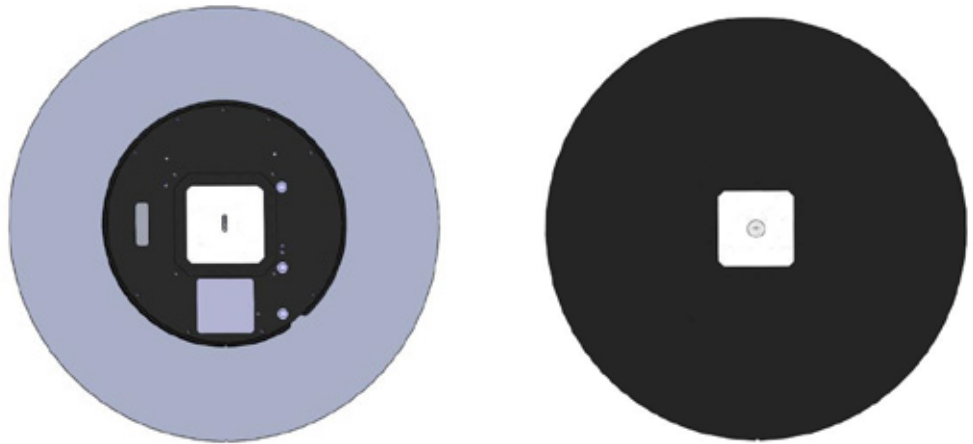
Figure 3 The new wafer-like sensor adds an upward looking camera to allow measurement and inspection of components above the sensor, such as showerheads and photoresist dispensing nozzles. Both upper and lower cameras are high-resolution, color cameras with white light illumination. The sensor is thinner and has a smooth bottom surface for better vacuum chucking. The ATS2 housing is constructed of chemically hardened glass and carbon fiber composite. The wafer shape conforms to the SEMI standards for 200mm and 300mm wafers regarding diameter and notch shape. The figure shows top (left) and bottom (right) views of a 300mm ATS2. The imaging optics are in the exact center of the wafer. The square white areas are the top and bottom illuminators.
