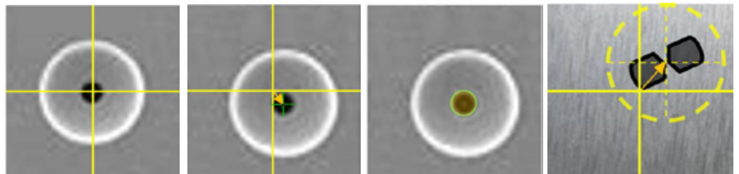
Figure 4 The new wafer-like sensor offers several operating modes: manual - the operator moves the alignment mark under a cross hair(left); assisted manual - the operator indicates the center of the alignment mark and the sensor calculates offsets (center left); automated - the operator selects a mark shape and indicates an approximate position, then the sensor finds the exact location and calculates offsets (center right); if provided a template, the automated mode can also be used with arbitrarily shaped marks (right).
