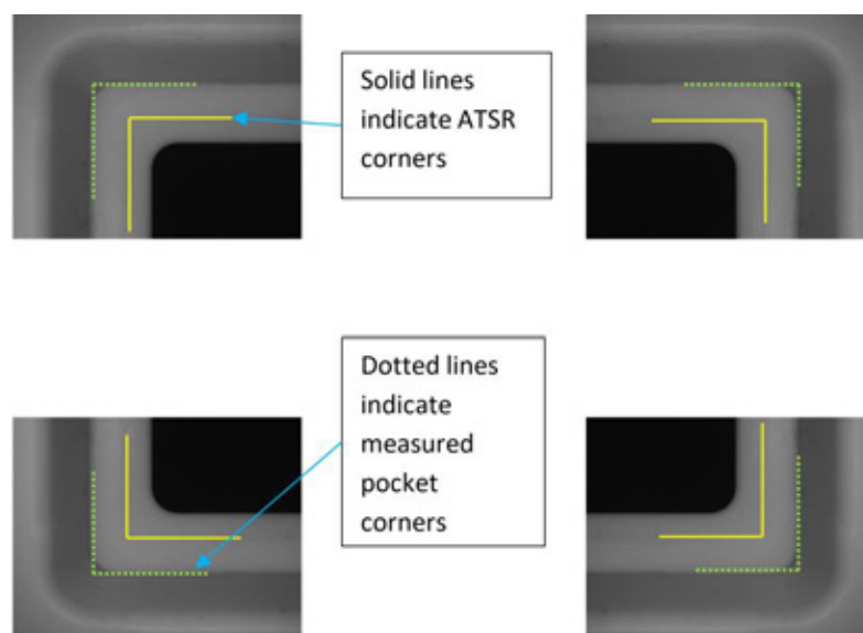
Figure 6 The reticle-like sensor presents images from cameras at each corner showing overlaid with marks to indicate the positions of the sensor corners (solid) and the extrapolated (squared off) pocket corners (dotted).
