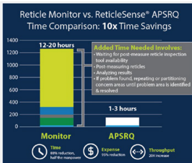
Figure 2 One comparison between conventional particle monitoring (cycling monitor reticles through the tool and counting the number of particles added) and particle counting using a reticle-like sensor reported up to 88% time savings, 95% reduction in costs, twenty times the throughput while requiring half the labor for the sensor-based approach.
