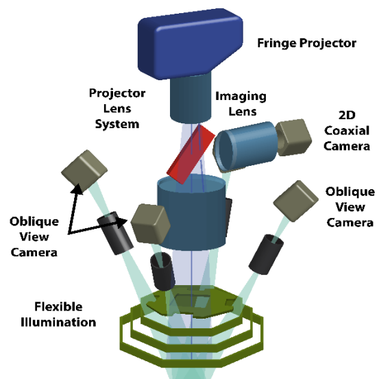
Figure 4 - The MRS sensor is designed specifically for 3D measurements. It uses a single top-down fringe projector coupled through an image splitter to a top-down 2D camera, and four oblique-view fringe cameras. The digital projector can generate fringes at multiple frequencies and orientations. The ability of the four oblique cameras to capture images in parallel significantly reduces image acquisition time.
