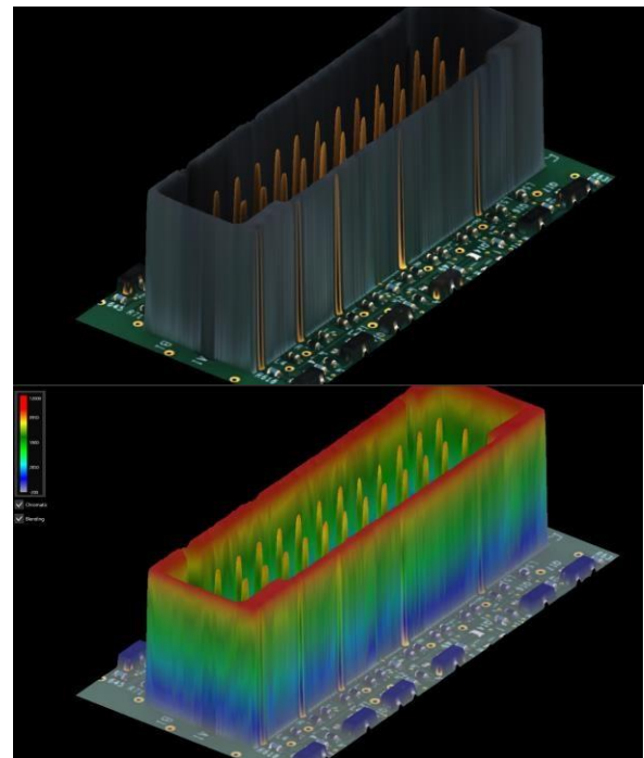
Figure 7 – MRS sensors can inspect and measure various assemblies with small components shadowed by tall
