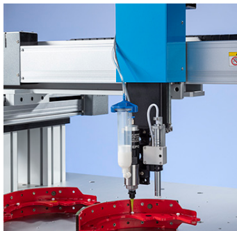
725D mounted on GV robot dispensing grease on automotive brake caliper.
