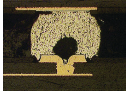
Figure 28. BGA Void Assessment: 17%, Inner Row, No fail, BGA256
