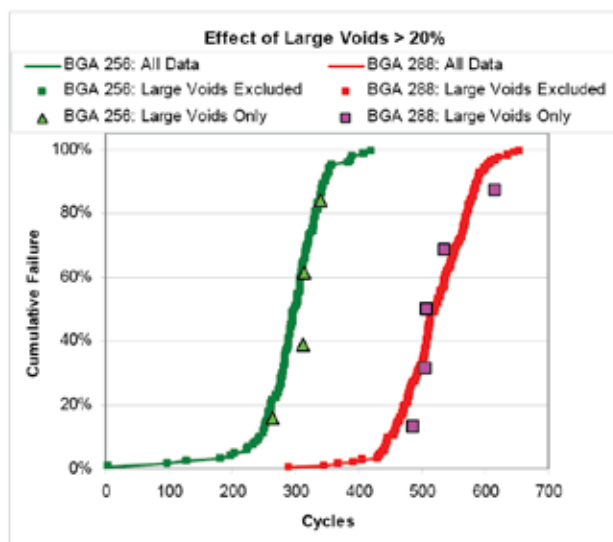
Figure 21. Effect of Large Voids Reliability Results
