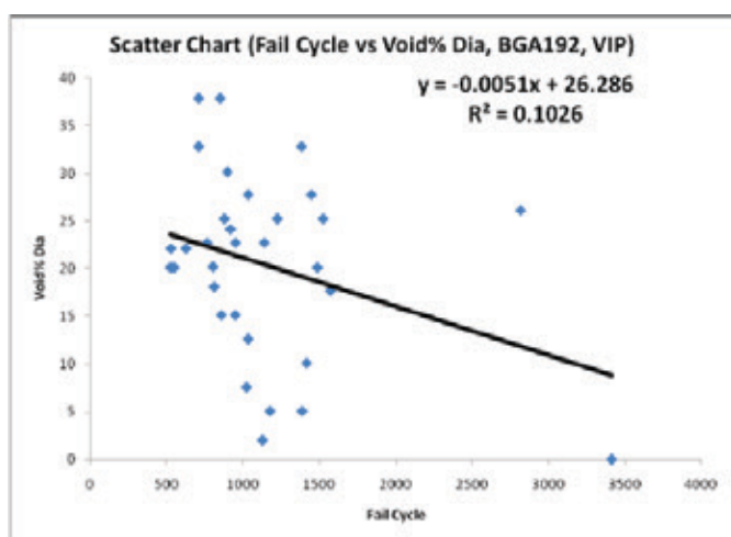
Figure 7. Scatter Chart Showing No Correlation between Solder Joint Void and Thermal Cycle Integrity, J. Smetana et al [10]
