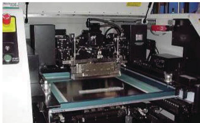
Figure 9. MPM Stencil Printer
