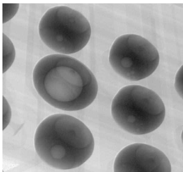
Figure 11. X-ray Examination of Test Vehicle Revealing: Top - Voids of 32% and 29% Area, Bottom - Oblique Angle X-ray View of 30% Void in BGA
