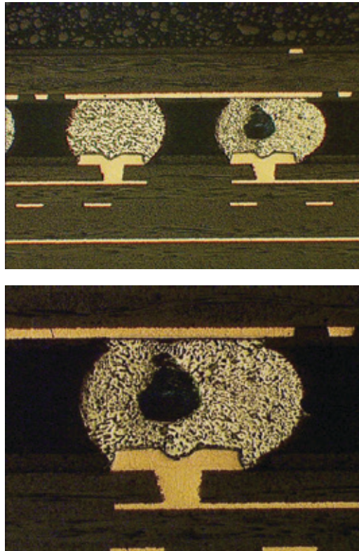
Figure 27. Macro (Top) and Magnified (Bottom) Views, BGA Void Assessment: 12%, Outer Row, No fail, BGA288
