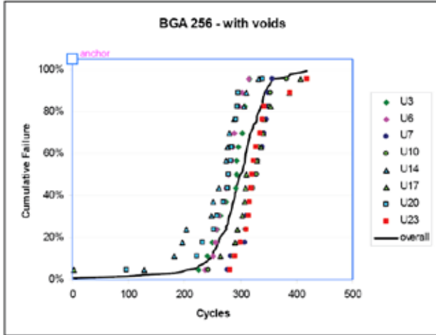
Figure 17. Failure Distributions by Reference Designator
