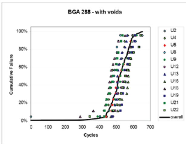
Figure 18. Failure Distributions by Reference Designator
