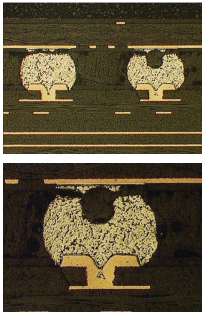
Figure 22. Macro (Top) and Magnified (Bottom) Views, BGA Void Assessment: 18% Void, Outer Row, 264 Cycles, BGA256
