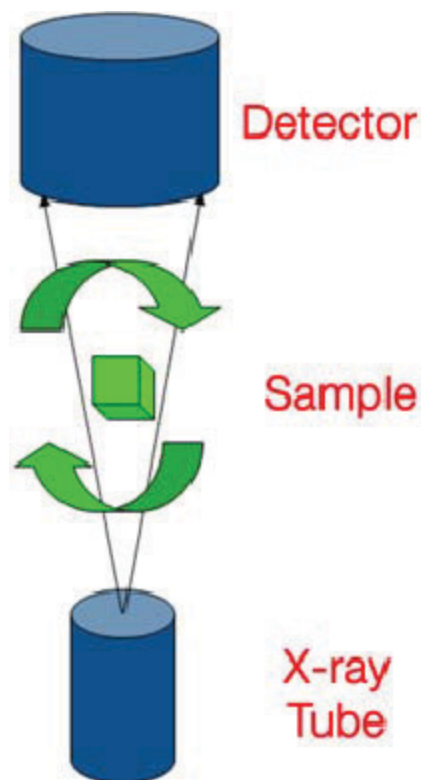
Figure 31. Schematic representation of the image acquisition phase of CT inspection
