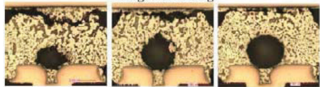
ENIG 2x Reflow – Examples of solder fatigue cracking without void interaction
