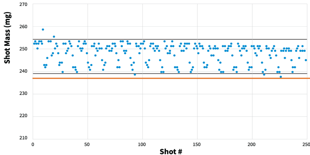
250mg Shot Mass Variation - ATS
