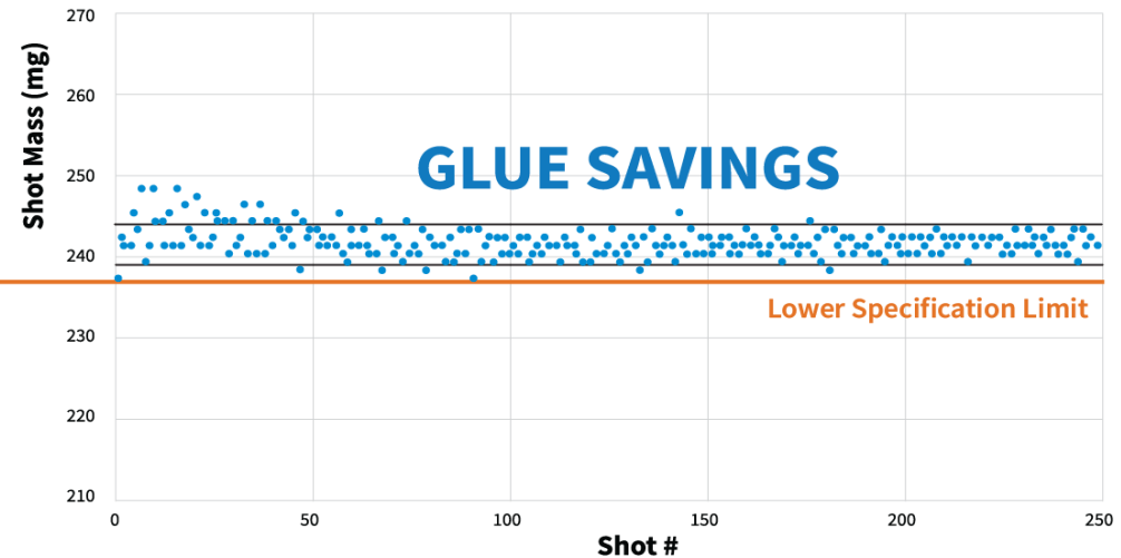
250mg Shot Mass Variation - ATS+ (with hydraulic regulator)
