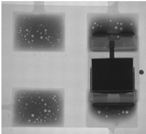
Figure 7: FR4 board material B with lead-free, vSAC alloy, solder paste 3.
