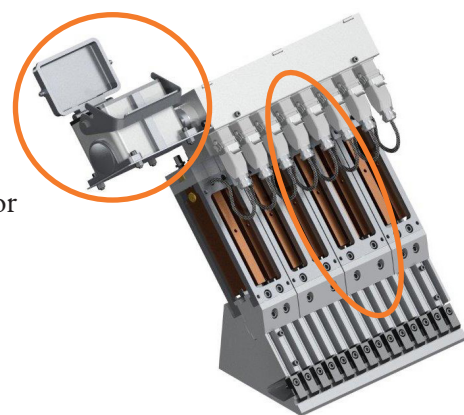
Autoflex™ VI-RE System: Close-up of Modules & Heater Wiring
